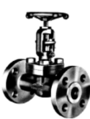
OS&Y globe integrally forged flanged ends class 300 and 600 bolted bonnet
